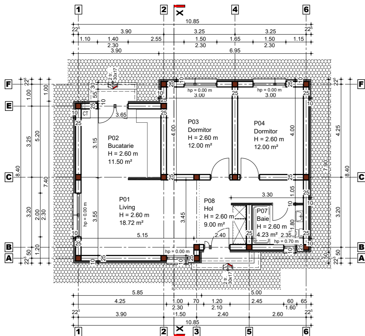
Plan Parter - corp C2 Sc. 1:100
