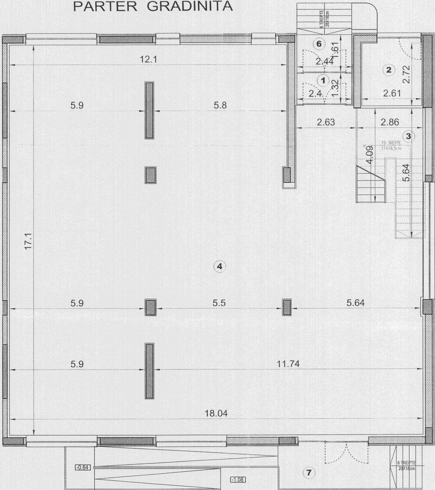
PARTER GRADINITA
