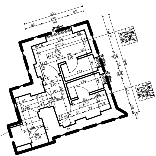
MEZANIN COTA +1.63
